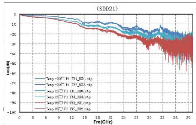
Temperature test data (26AWG 3M)
