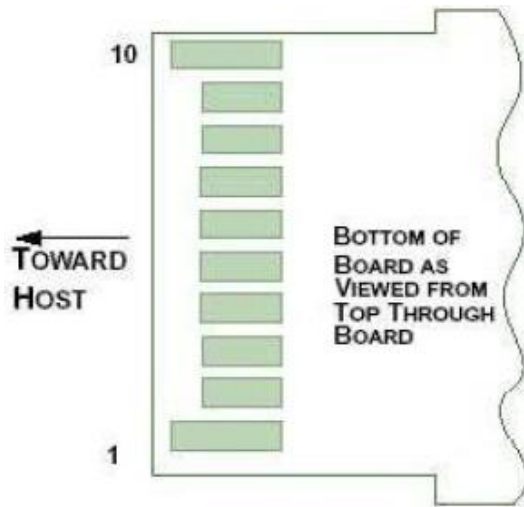
Figure 1s: MSA Compliant Connector
