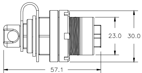
SUPERTAP/SCX ADAPTER
