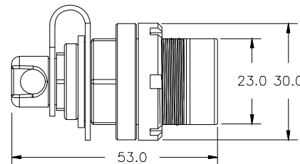
SUPERTAP/MPOX ADAPTER
