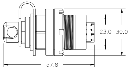
SUPERTAP/LCX ADAPTER
