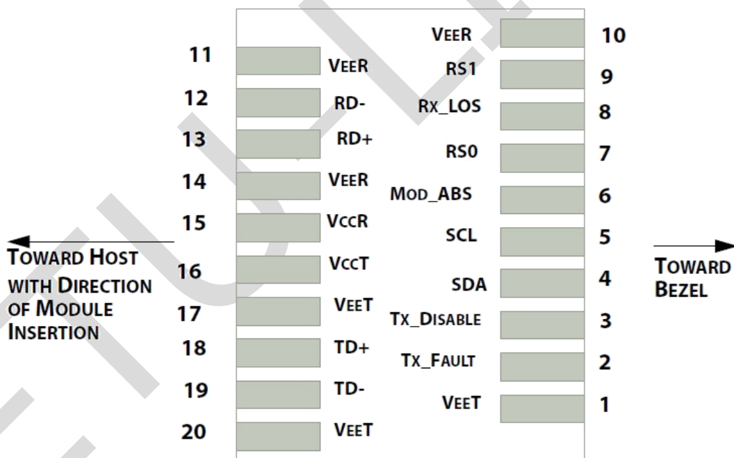
Figure 2: Pin Definitions compliant
