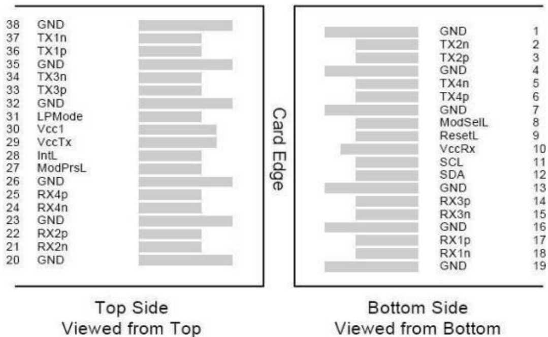
Figure 2: Pin Definitions
