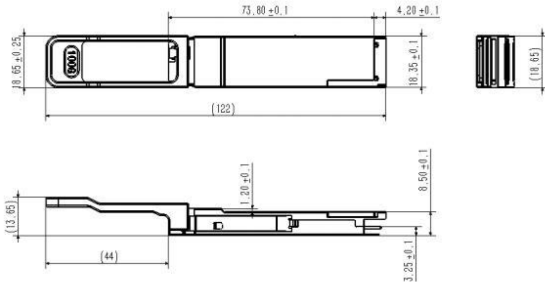
Figure 5. Mechanical Schematic
