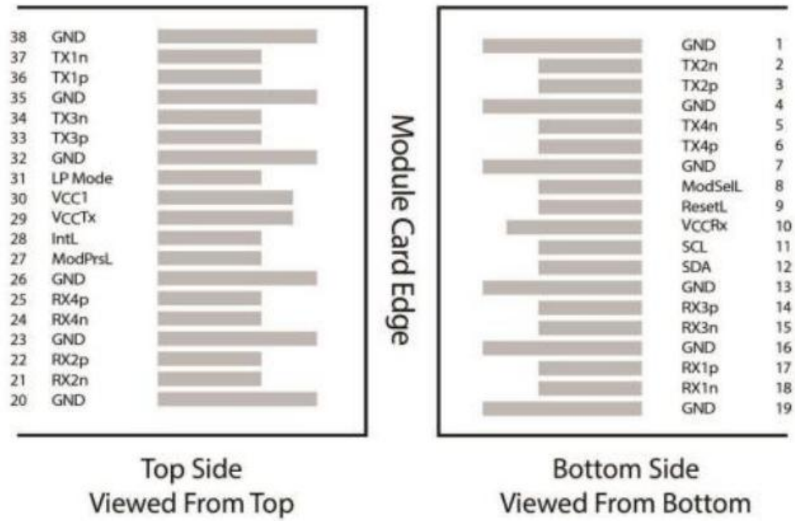
Figure 2. QSFP28 Connector Pad layout
