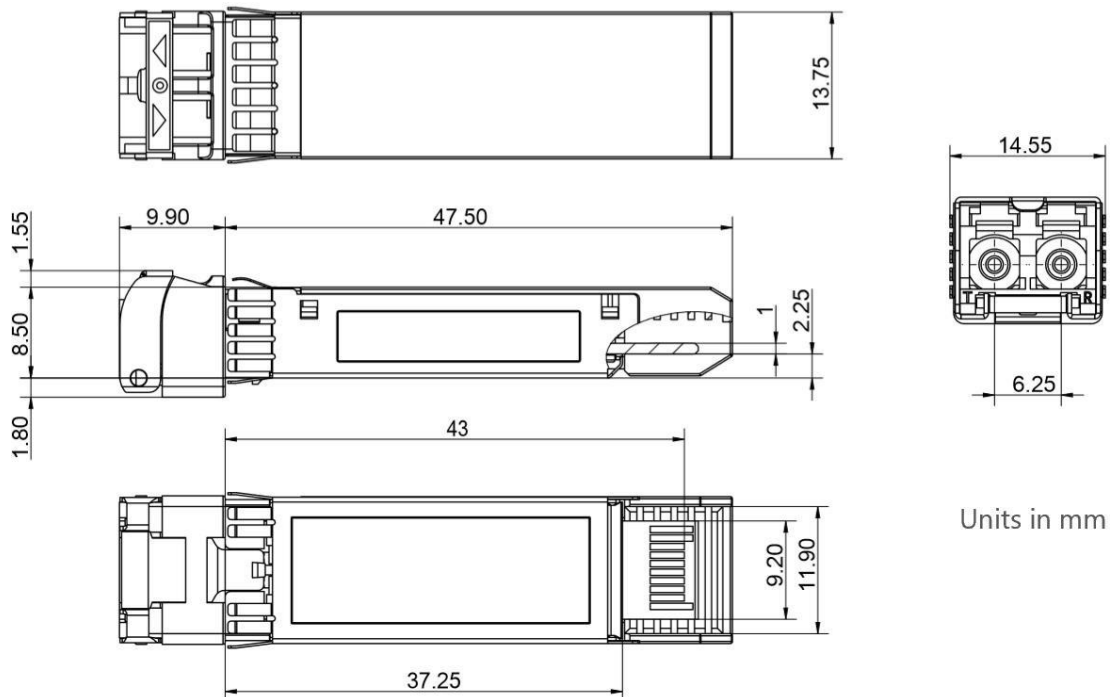
Figure2. Mechanical Outline
