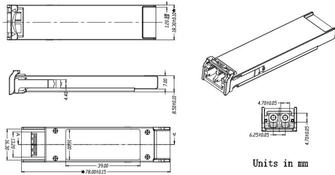
Figure2. Mechanical Outline
